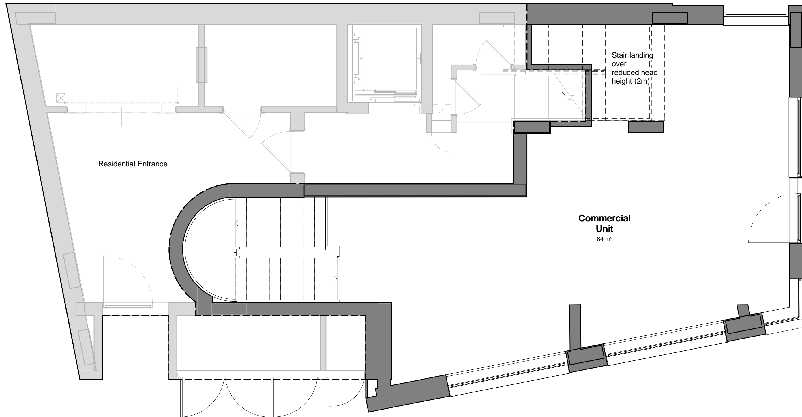
1 G00 - Ground Floor Plan 1 : 50
